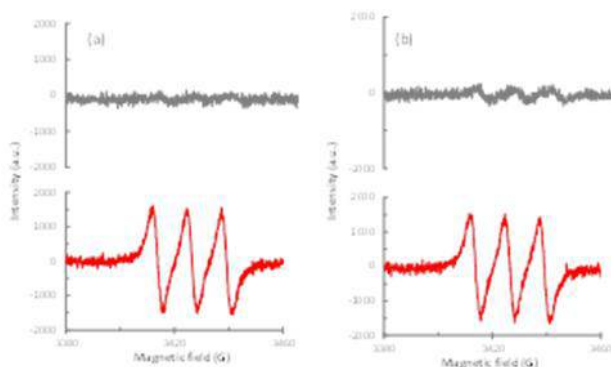
Triplet electron paramagnetic resonance signals from NO trapping by [Fe(MGD) 2 ] for trans -(Cl,Cl)-[Ru(FT)Cl 2 (NO)]PF 6 (a) and cis -(Cl,Cl)-[Ru(FT)Cl 2 (NO)]PF 6 (b) upon two-photon excitation at \lambda = 810 nm. Control (black line) before irradiation.
