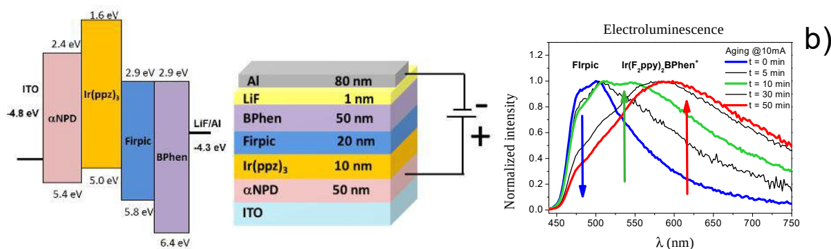
Figure 1: a) Proposed chemical degradation of Flrpic emitter; b) OLED structure (αNPD: hole transport material; Ir(ppz) 3 : electron blocking layer) and material energy levels; electroluminescence spectral change during OLED aging.
