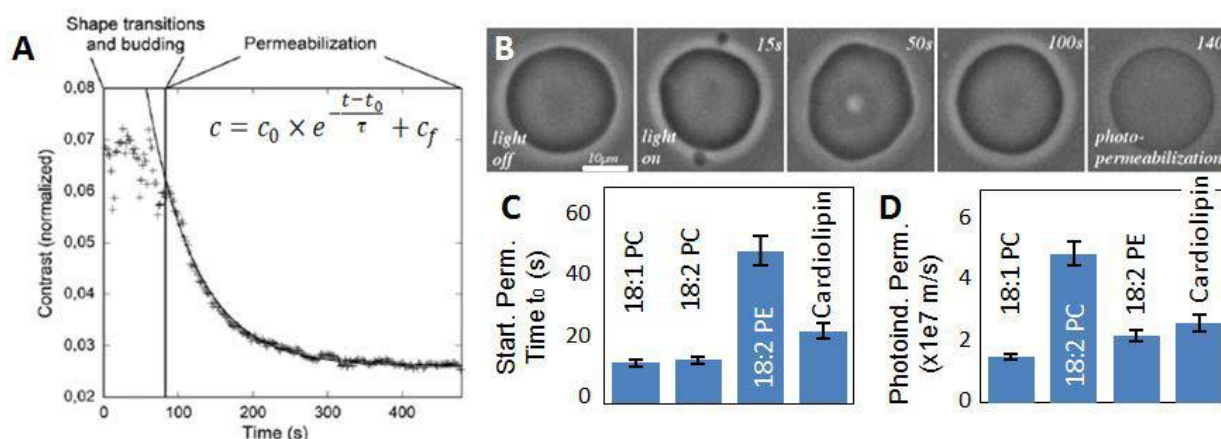
(a-b) Typical exponential decrease of a being-oxidized vesicle contrast. (c-d) Starting permeation time and photo-induced permeability for different membrane composition.
